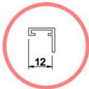
DETAIL A' (LMT-MINI frame)
